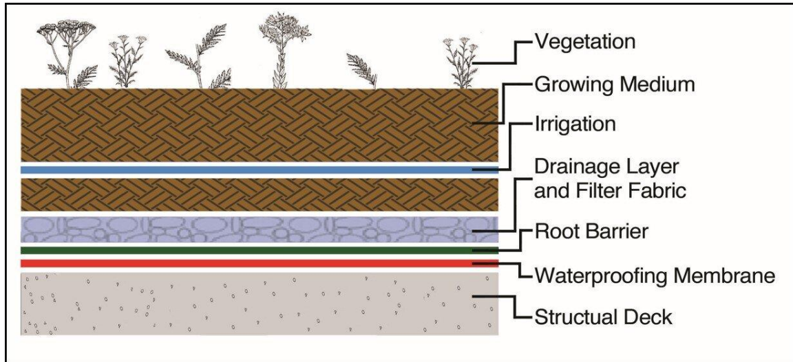
Figure 11.5-4: Typical green roof cross-section (with optional irrigation) (guideline 4b).
